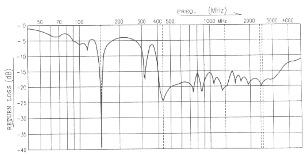
DS3000A FREQUENCY CHARACTERISTIC
